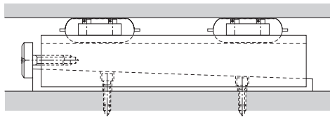
(c) Adjusting a tapered gibe
