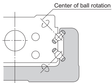
Fig.4 Contact Structure of Model KR
