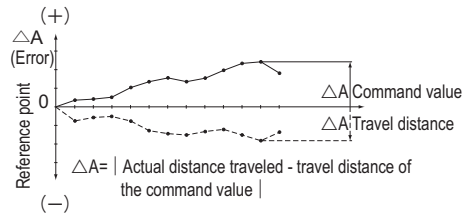
Fig.10 Positioning Accuracy
