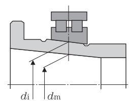
Fig. 6.21 Explanation of d_m/d_i
